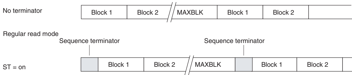
Figure 5-2. Read Data Stream with Sequence Terminator
